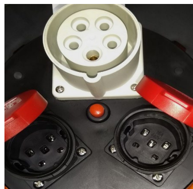
Kabelrolle KRPCEE16/5 IP44 / IP55 = CH T25 / Kabel Pur orange H07BQ-F 5x2,5mm 2
